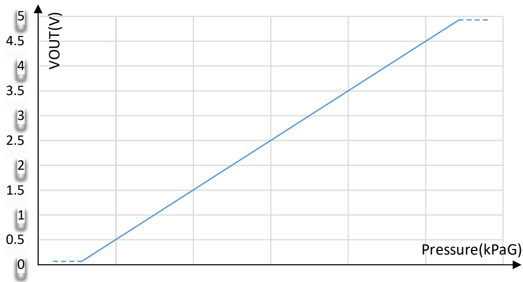
Fig 5.2 Analog Output Transfer Function
