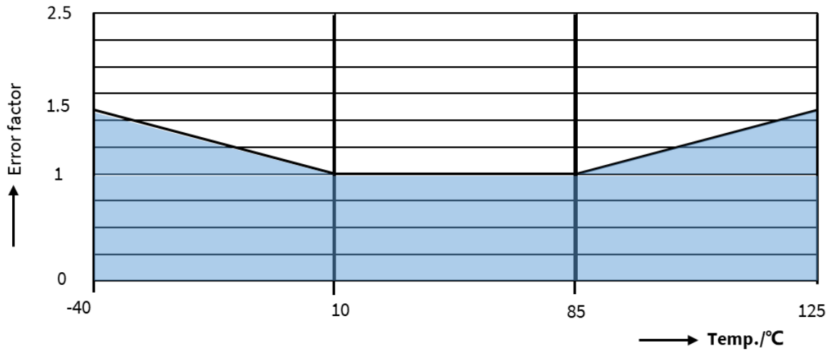
Fig 5.4 Accuracy for Pressure Acquisition
