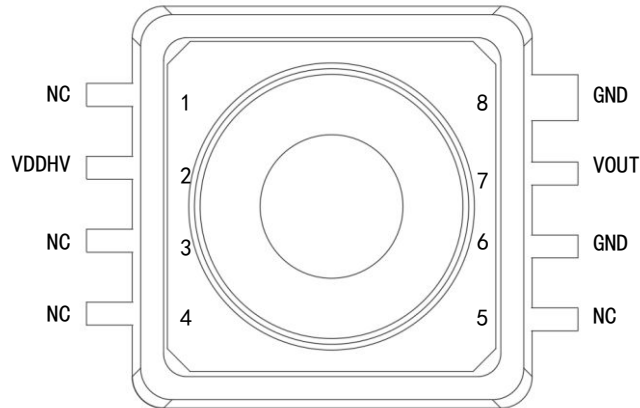
Fig 1.1 Pin Definition (Top view)
