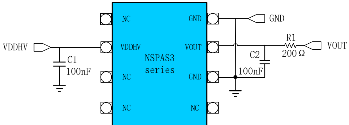
Fig 6.1 Application Circuit
