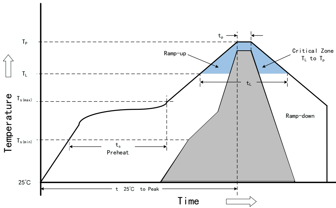
Fig 6.3 Soldering Profile
