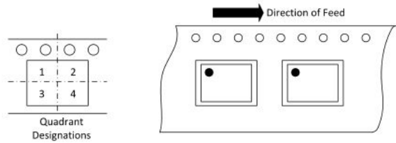
Figure 12.1. tape and reel information for TSSOP24
