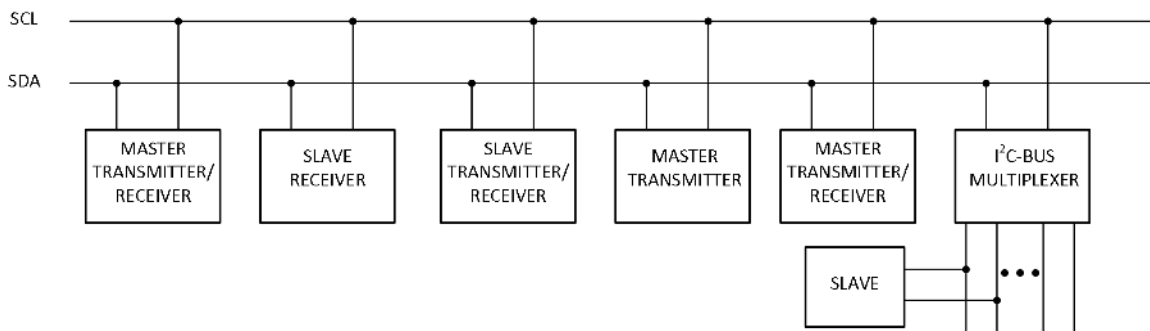
Figure 8.3. System configuration
