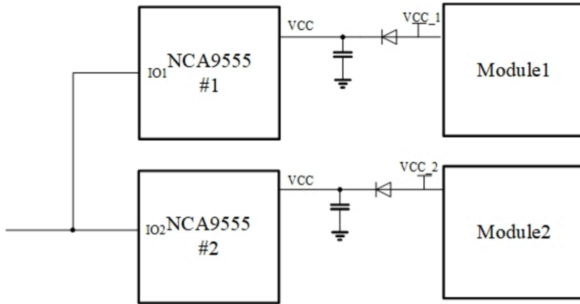
Figure 9.2. Typical application
