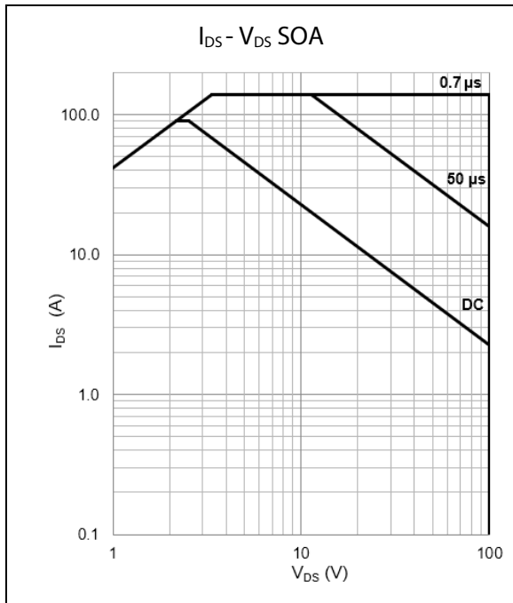
Figure 13: Safe Operating Area @ T_{case} = 25\text{ }^{\circ}\text{C}
