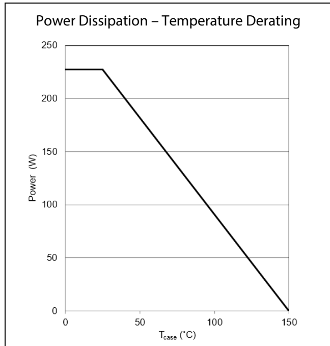
Figure 14: Power Derating vs. T_{case}
