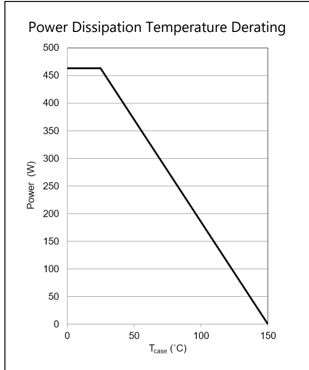
Figure 14: Power Derating vs. T_{case}
