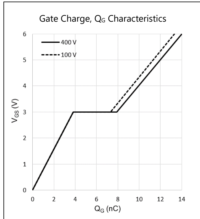
Figure 6: Typical V_{GS} vs. Q_G @ V_{DS}=100, 400\text{ V}
